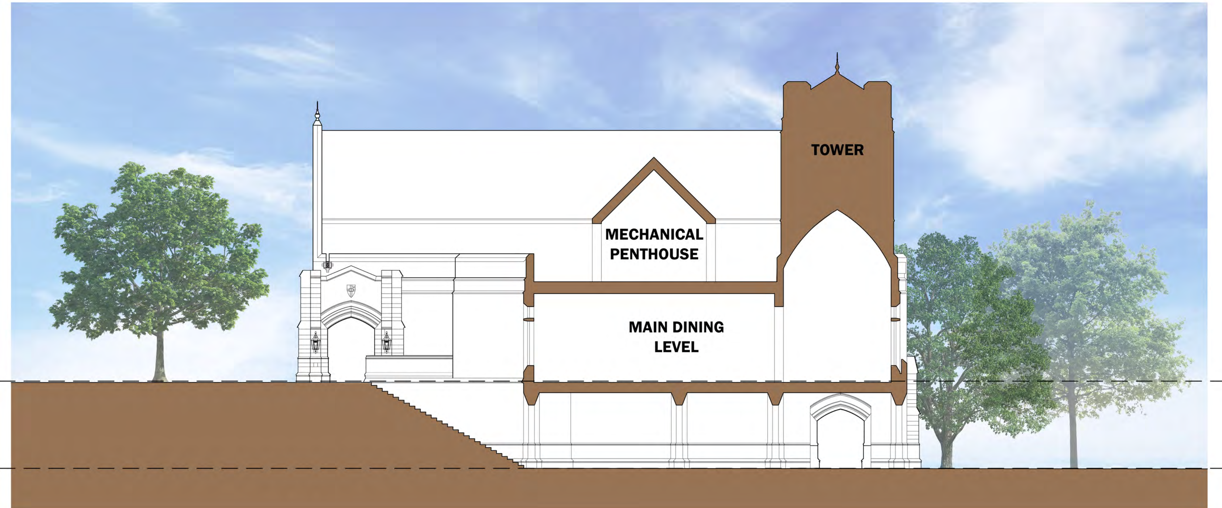
SECTION A
